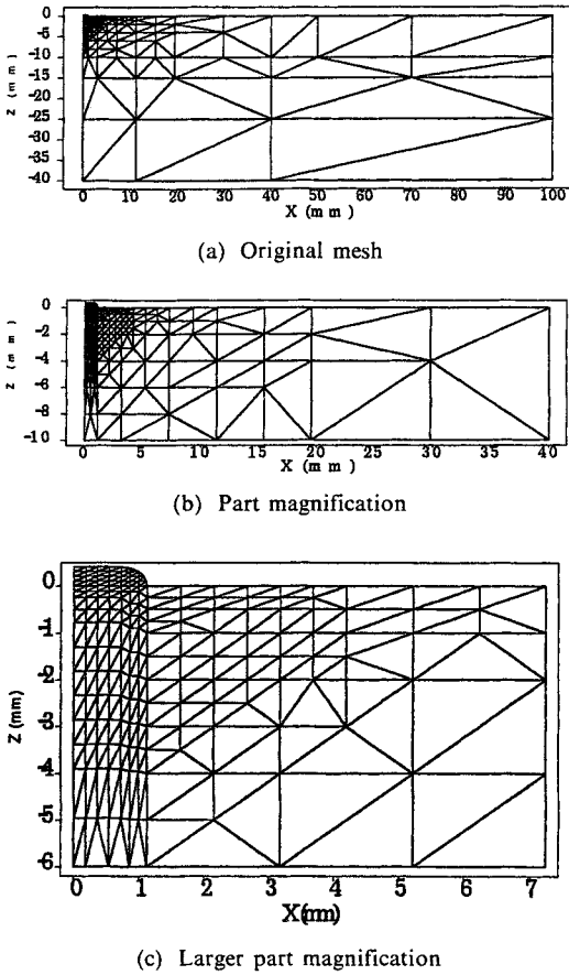
Fig. 2 Original mesh
