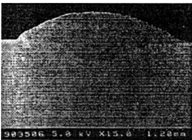
(c) Cladding speed=2mm/s, 25mm away from the beginning
