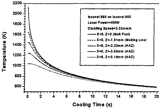
(a) Temperatures during cooling
