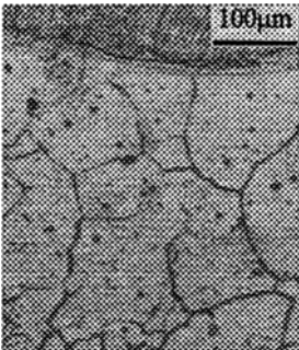
(c) Cladding speed=1mm/s, 25mm distance from the beginning
