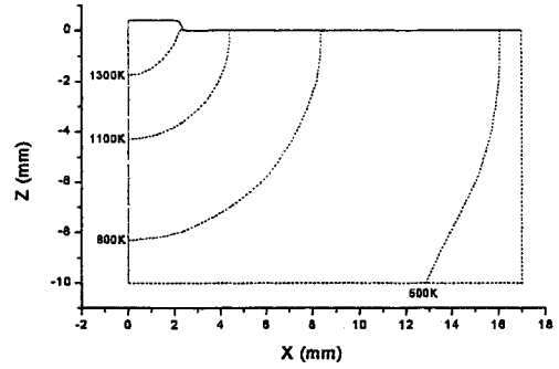
(b) Thermal field after 1.06s cooling
