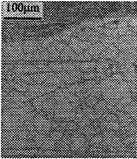
(a) Cladding speed=2.5mm/s, 25mm distance from the beginning
