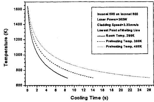
(b) Temperatures during cooling
