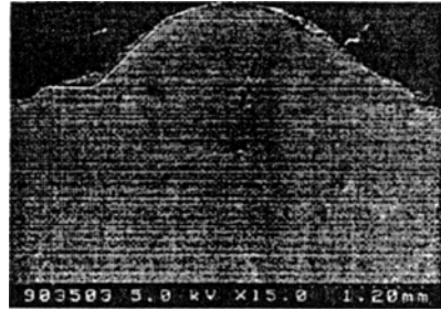
(b) Cladding speed=1.5mm/s, 25mm away from the beginning
