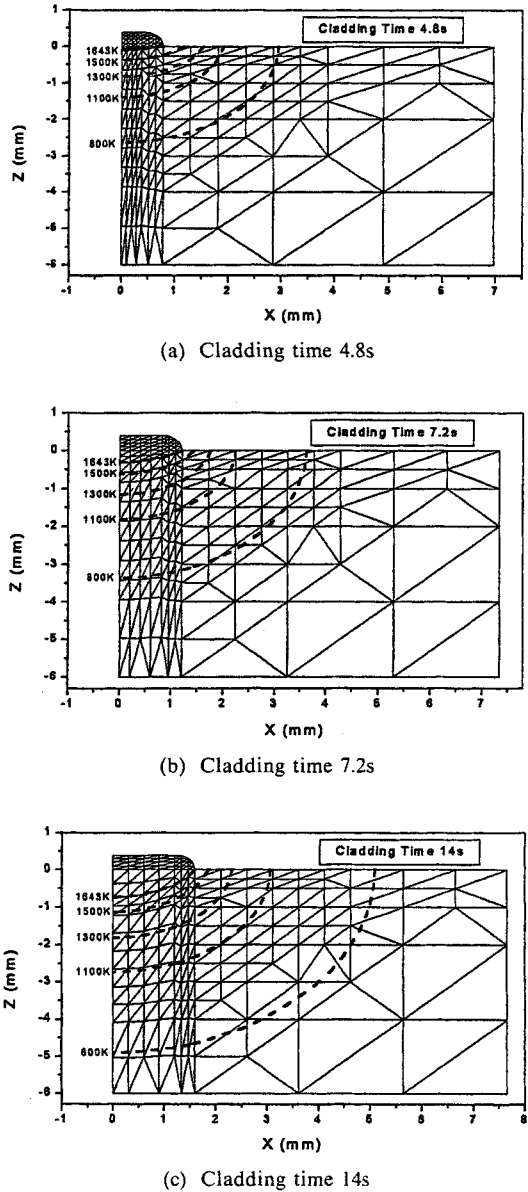
Fig. 3 Meshes and thermal fields at different cladding times
